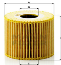
Oil Filter HU 819 x EM-10147
