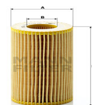
Oil Filter HU 719/8 x EM-10143
